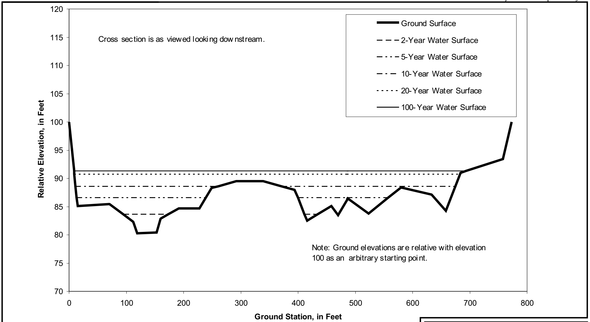
Simulation Of Natural Flows In Middle Piru Creek Project Figure 3.2-16 Cross Section L3 With-Project Water Surface Elevations
